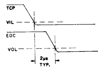
Fig.41 EOC TURN-OFF
